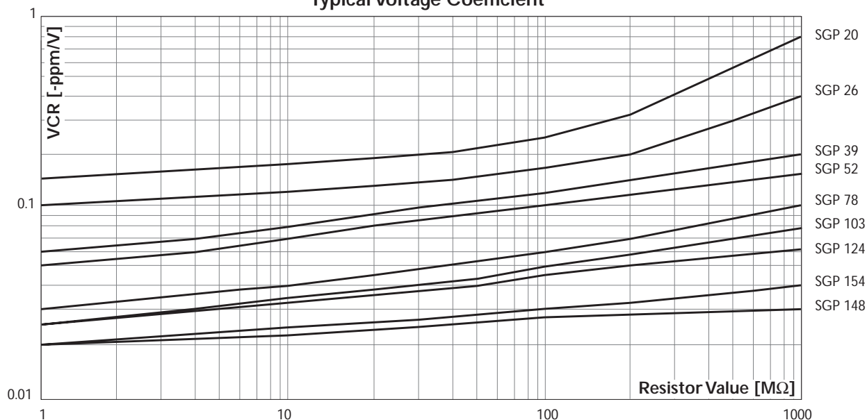
Typical Voltage Coefficient
